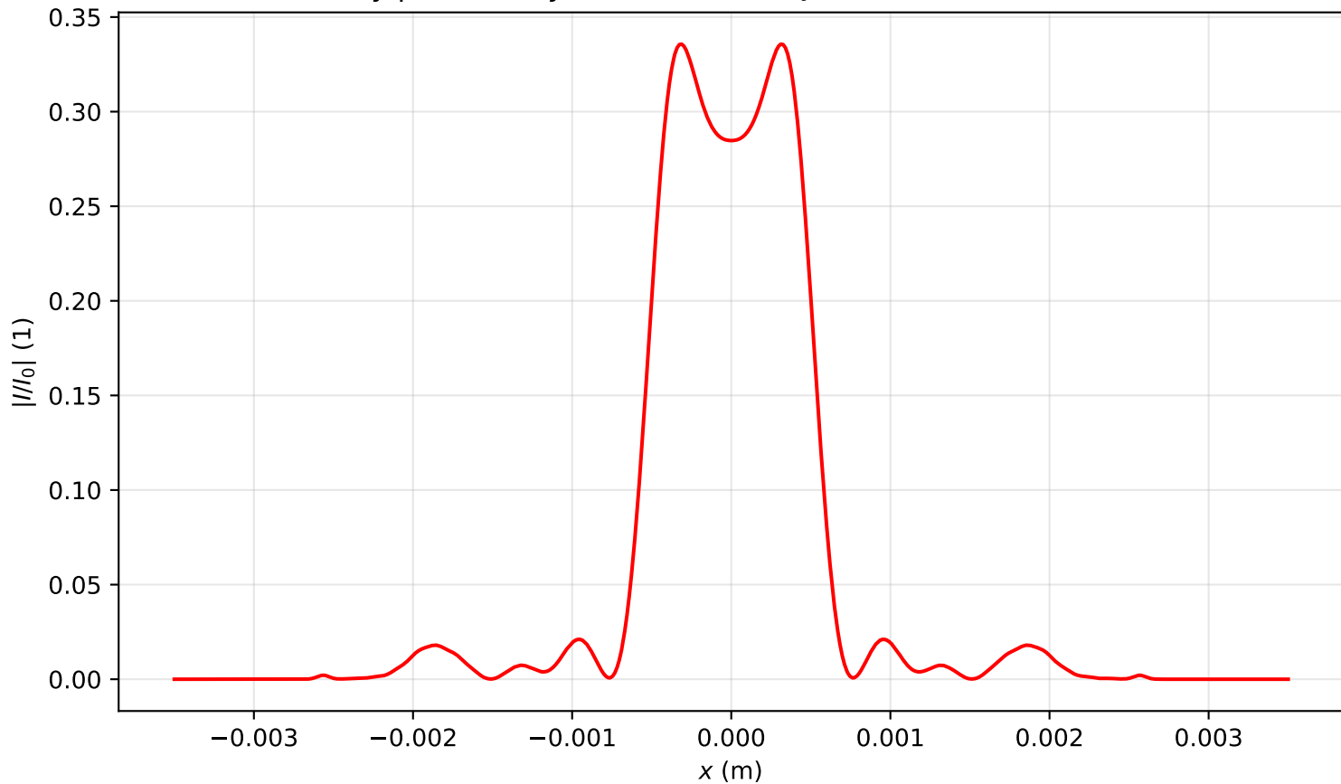
Intensity profile I(x, y = 0, z = 0.796)/I_0 , P_{in}=3.0P_{cr} , artificial time
